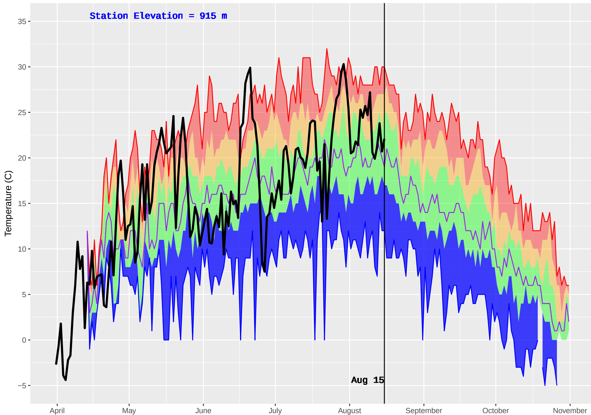
MCLEOD LAKE (153) : Historical (1990–2016) and Current (2018) Daily Temperature
