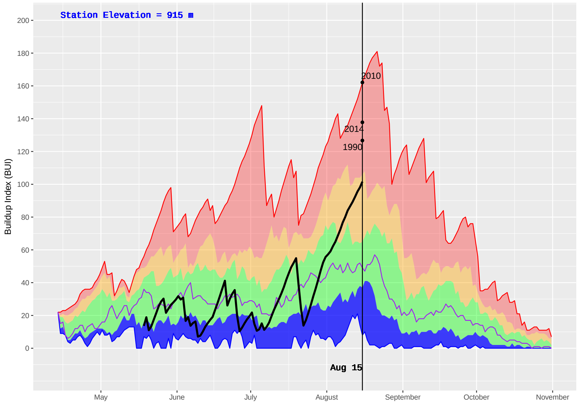
MCLEOD LAKE (153) : Historical (1990–2016) and Current (2018) Daily Buildup Index (BUI)
