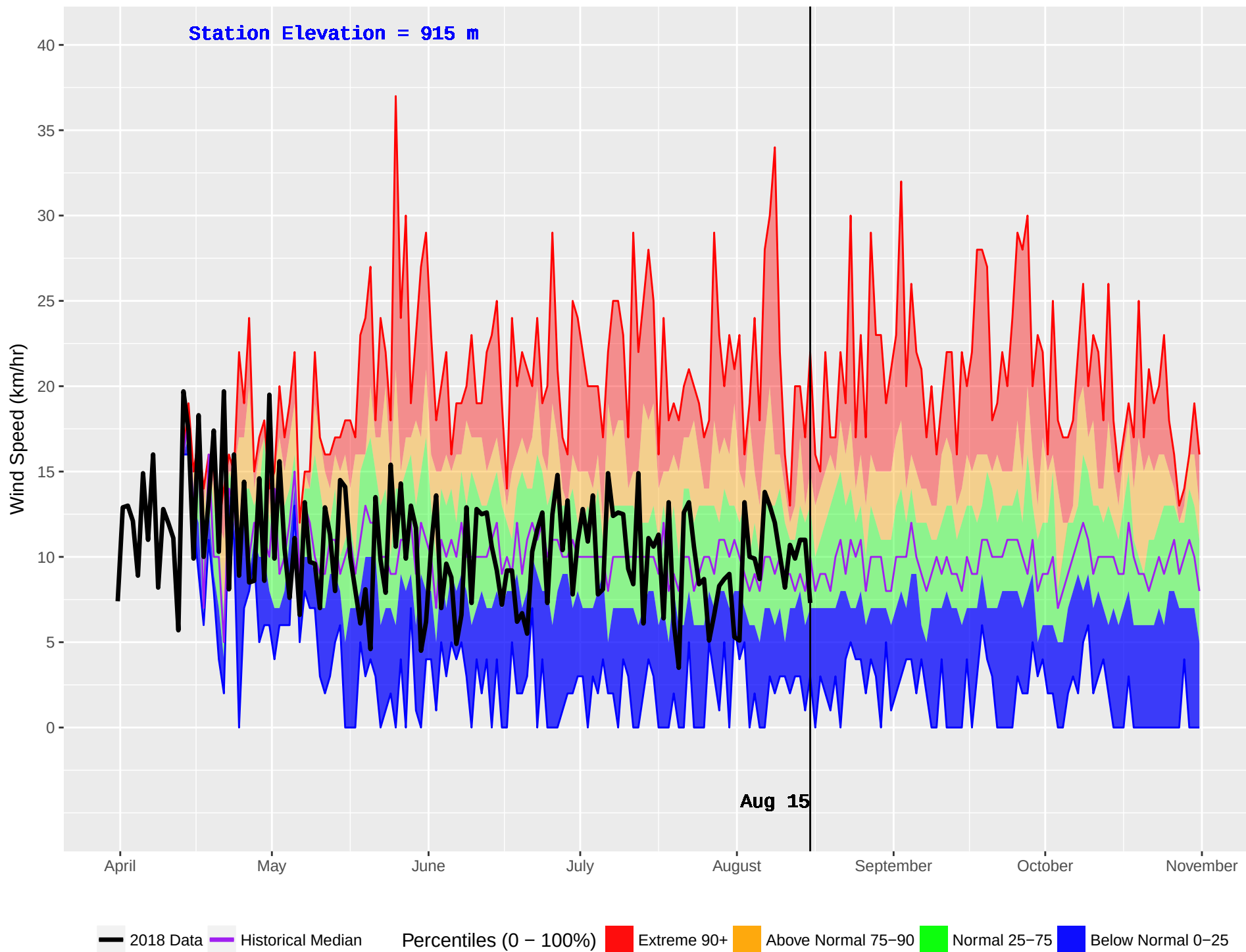
MCLEOD LAKE (153) : Historical (1990–2016) and Current (2018) Daily Wind Speed
