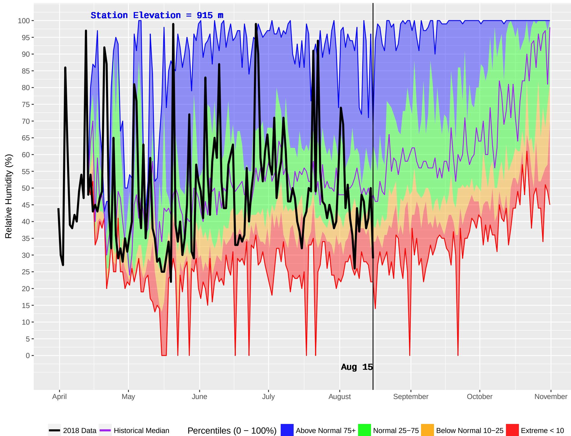
MCLEOD LAKE (153) : Historical (1990–2016) and Current (2018) Daily Relative Humidity
