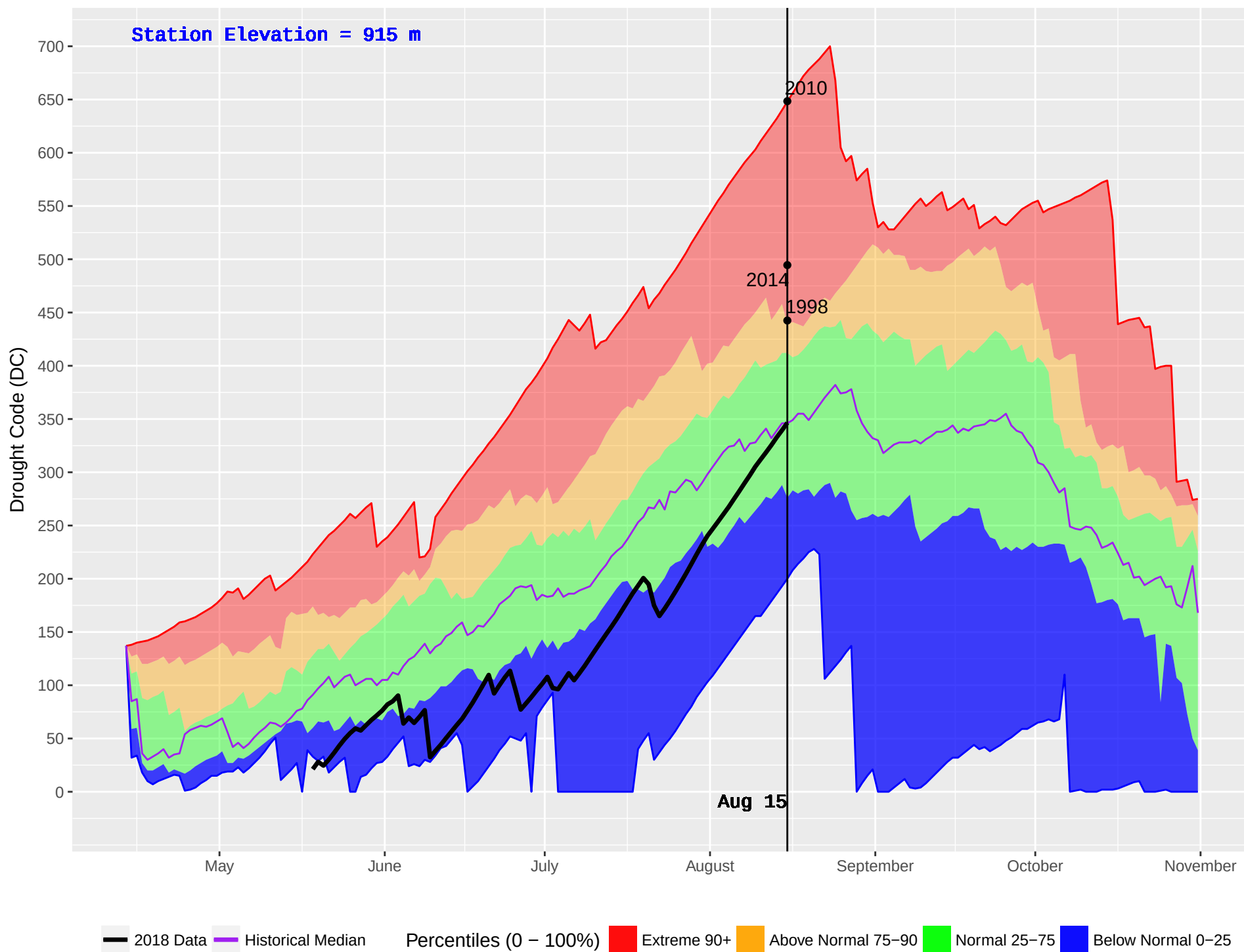
MCLEOD LAKE (153) : Historical (1990–2016) and Current (2018) Daily Drought Code (DC)
