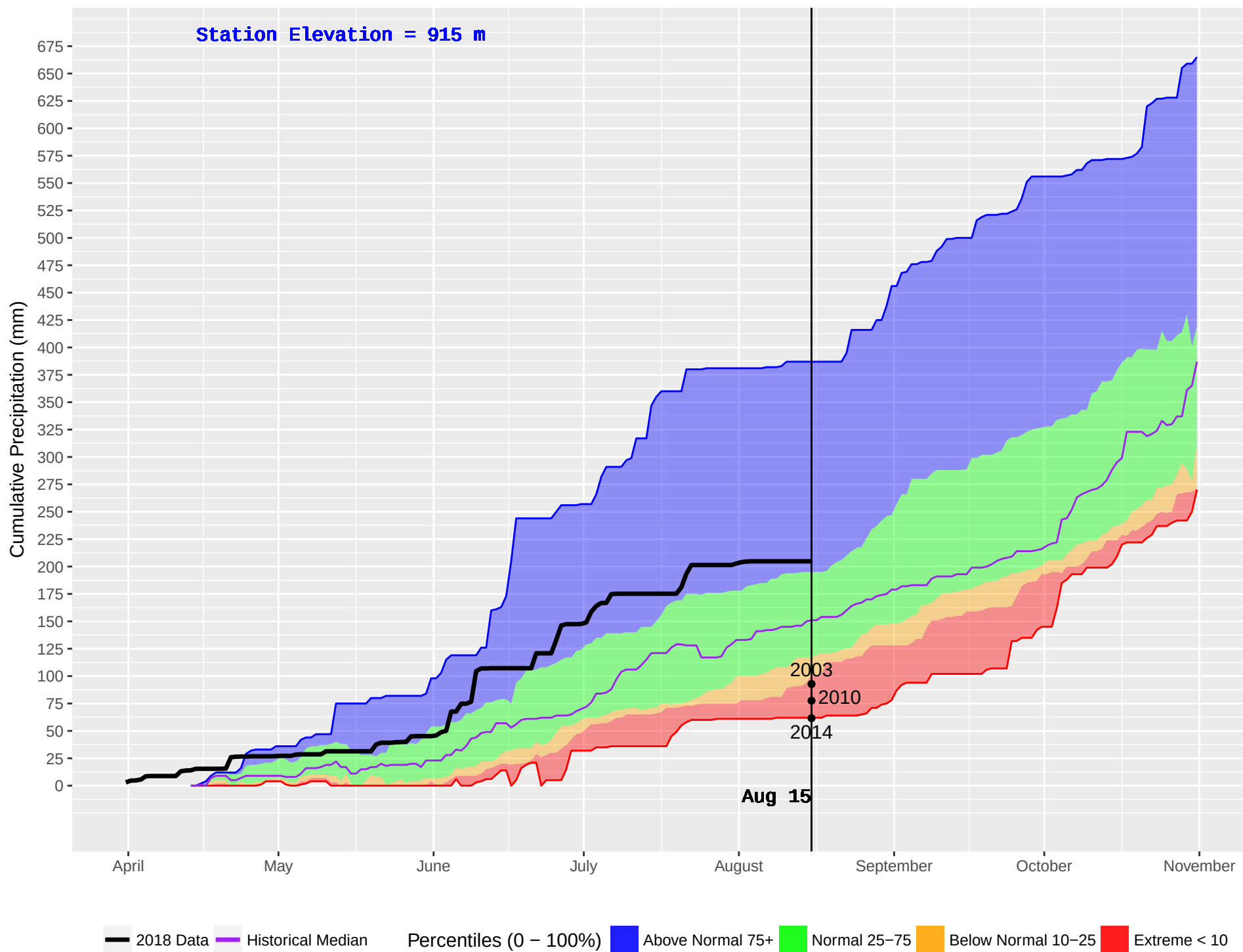
MCLEOD LAKE (153) : Historical (1990–2016) and Current (2018) Daily Cumulative Precipitation
